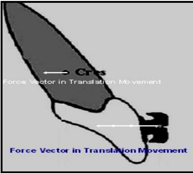
Figure 1: The force vectors in case of translation movement of the anterior teeth.
