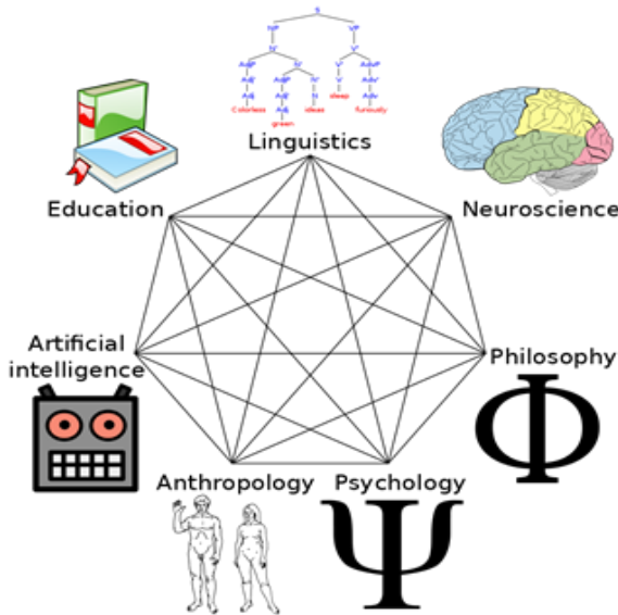
Figure 1: Cognitive science.
