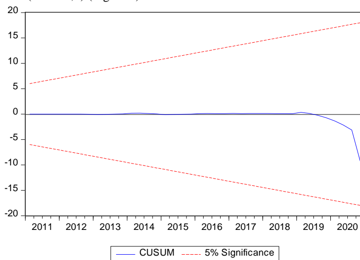
Figure 1: Stability test - plots of cumulative sum of residual.
